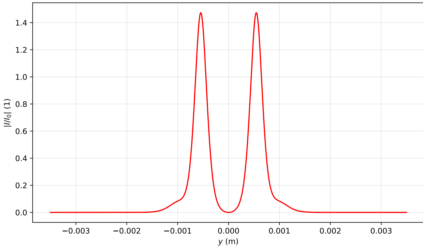
Intensity profile I(x=0, y, z=0.637)/I_0 , \text{Pin}=7.0\text{Pcr} , artificial time
